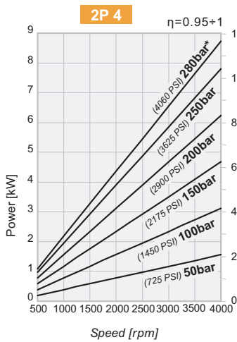
Pumps Group 2 Power and Speed Diagrams
