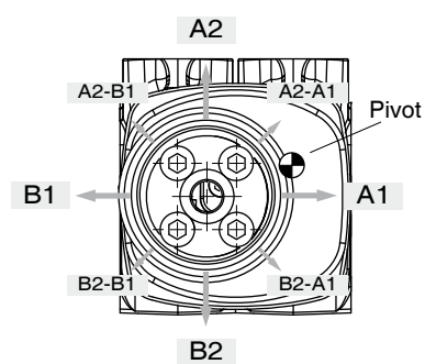
LCB4 configuration with pivot placed above on the right
