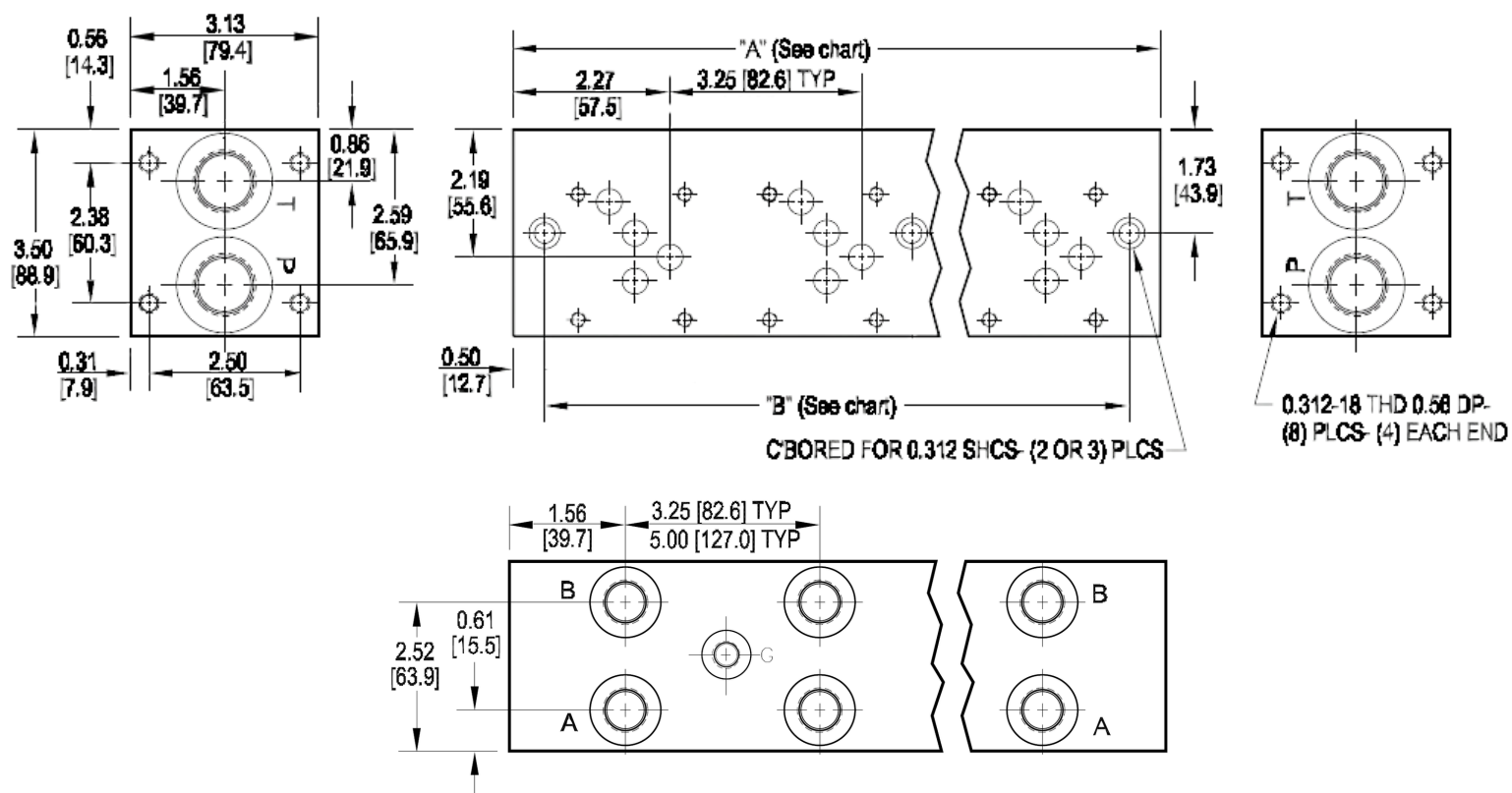
Parallel Circuit with Cavity and Gauge Port
