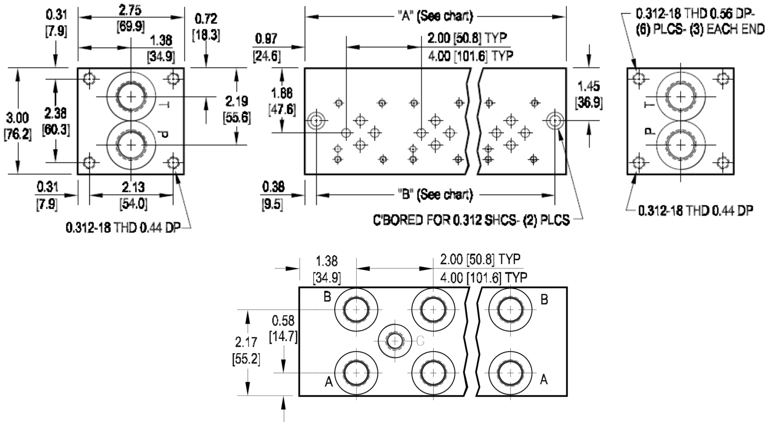
Parallel Circuit with Cavity and Gauge Port
