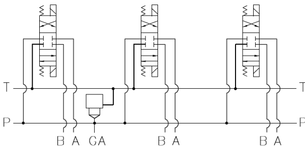
Parallel Circuit with Cavity and Gauge Port
