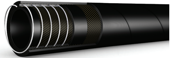
RBR-12 19mm (0.75 in) DN19 21 bar (305 psi) SAE100R4
