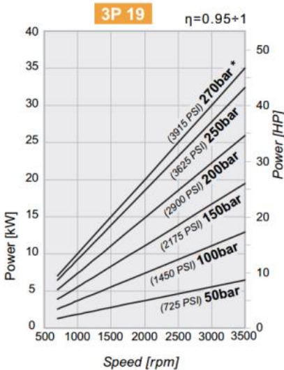
Pumps Group 3 Power and Speed Diagrams
