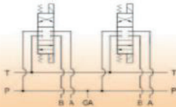
Parallel Circuit
