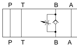
DGMFN-5-Y-B**-30
