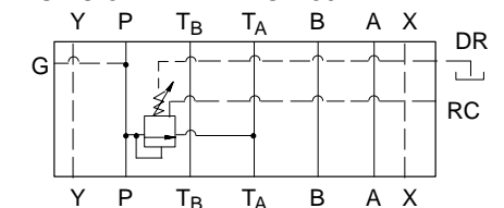
DGMC-5N-PT-**-E-RC-**-30
