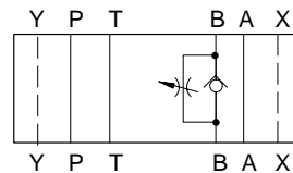
DGMFN-5N-Y-B**-30
