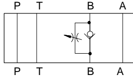
DGMFN-5-X-B**-30
