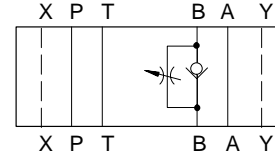
DGMFN-5P-X-B**-30
