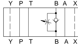
DGMFN-5N-X-B**-30
