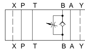
DGMFN-5P-Y-B**-30
