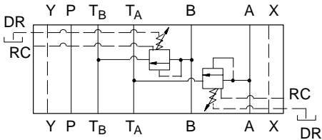
DGMC2-5N-AT-**-E-BT-**-E-RC-**-30
