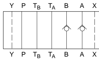
DGMDC-5N-Y-A*-B*-30
