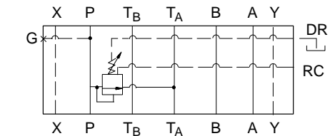
DGMC-5P-PT-**-E-RC-**-30
