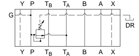
DGMC-5N-PT-**-E-**-30
