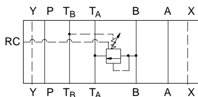
DGMC-5N-BT-**-RC-**-30
