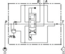
Hydraulic Symbol
