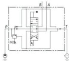
Hydraulic Symbol
