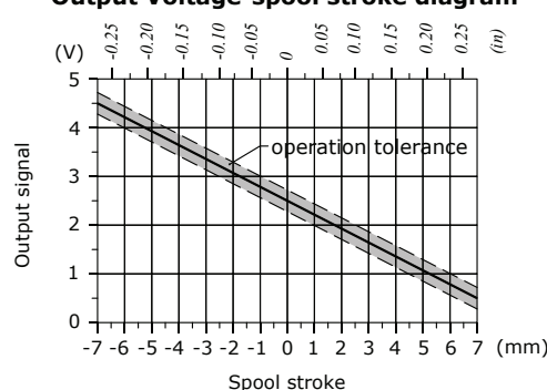
Output Voltage-spool stroke diagram
