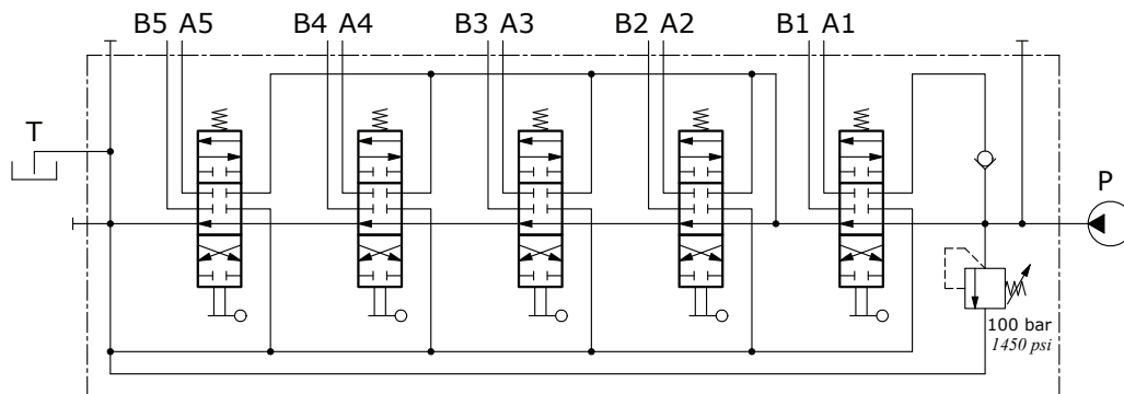
Description example 90L GM10/5- SP 4(X-100)/ED-18L/ED-18L/ED-18L/ED-18L/AET-PSL4
