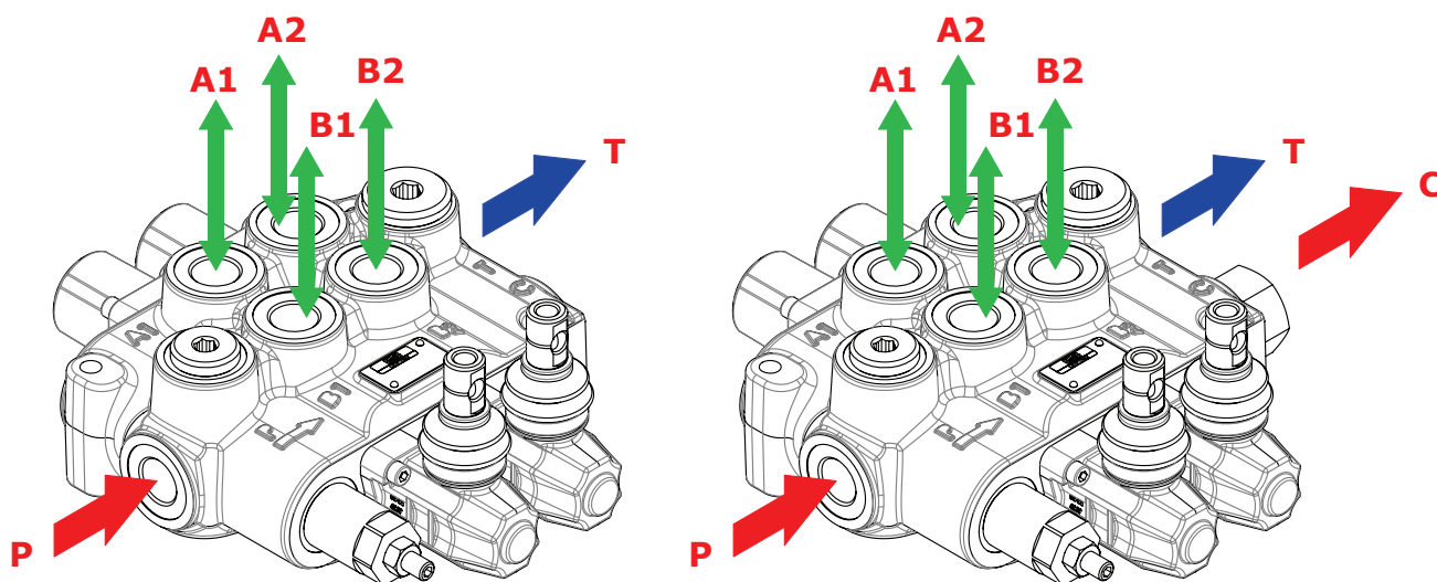
Carry-over configuration
