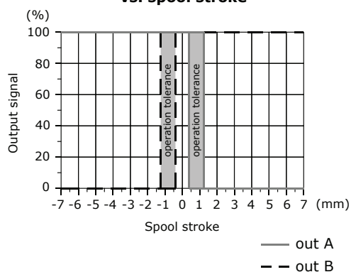
Output signal (SPSD example) vs. spool stroke
