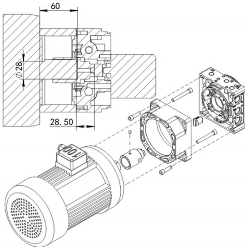
Aluminum Flange: 560100
