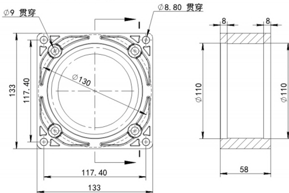
Aluminum Flange: 560100
