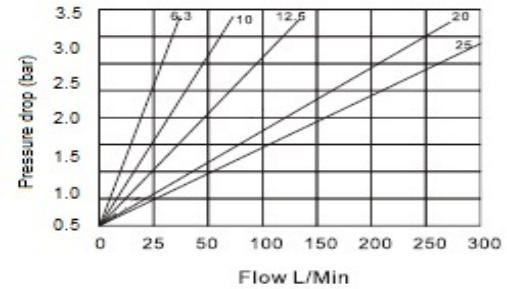
FLOW CURVE/PRESSURE DROP
