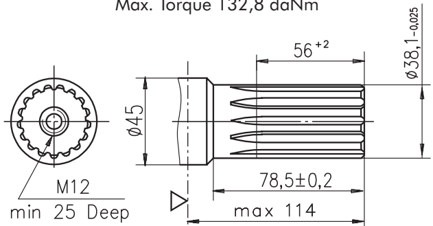
SH - \phi 1\frac{1}{2} " splined 17T, DP 12/24 ANSI B92.1-1976 Max. Torque 132,8 daNm
