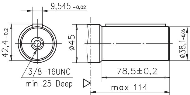
CO - \phi 1\frac{1}{2} " straight, Parallel key \frac{3}{8} "x \frac{3}{8} "x 2\frac{1}{4} " BS46 Max. Torque 132,8 daNm
