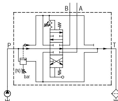
Hydraulic Symbol
