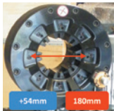
Large die opening = 180mm Radial die travel = + 54mm
