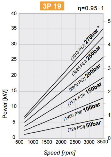
Pumps Group 3 Power and Speed Diagrams
