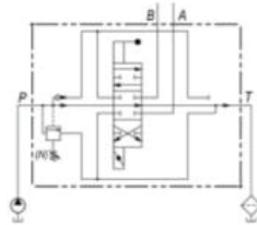
Hydraulic Symbol
