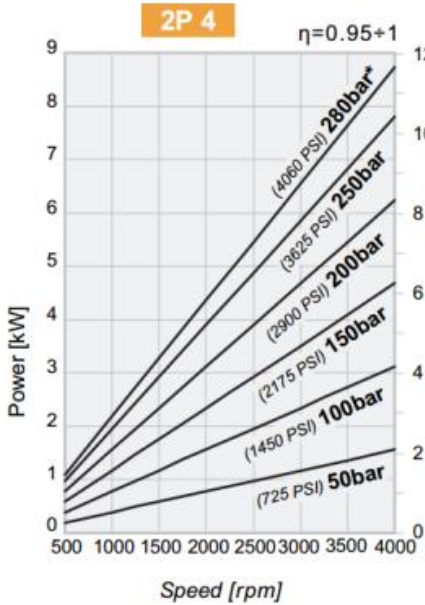
Pumps Group 2 Power and Speed Diagrams
