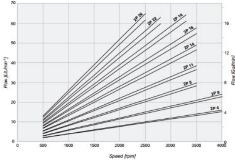
Flow - Speed chart
